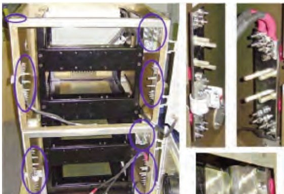
Chassis showing application of Plastic SurLok
